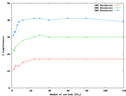
Figure 7: Pattern Time Periods
