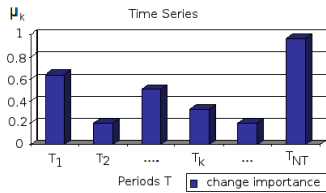
Figure 2: Time Series
