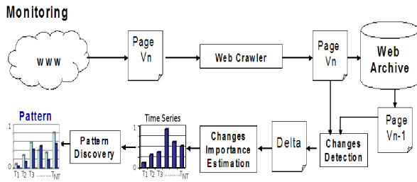
Figure 3: Pattern Discovery Framework
